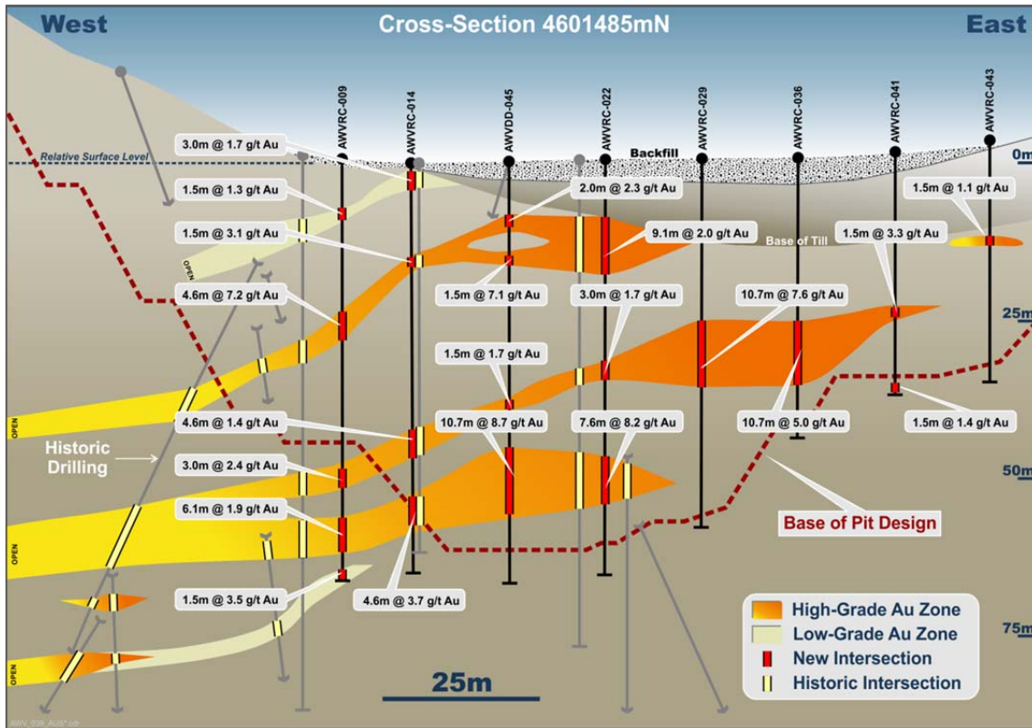
Figure 5: Cross section 4601485mN showing new drilling results at the 601 zone, South Sammy
