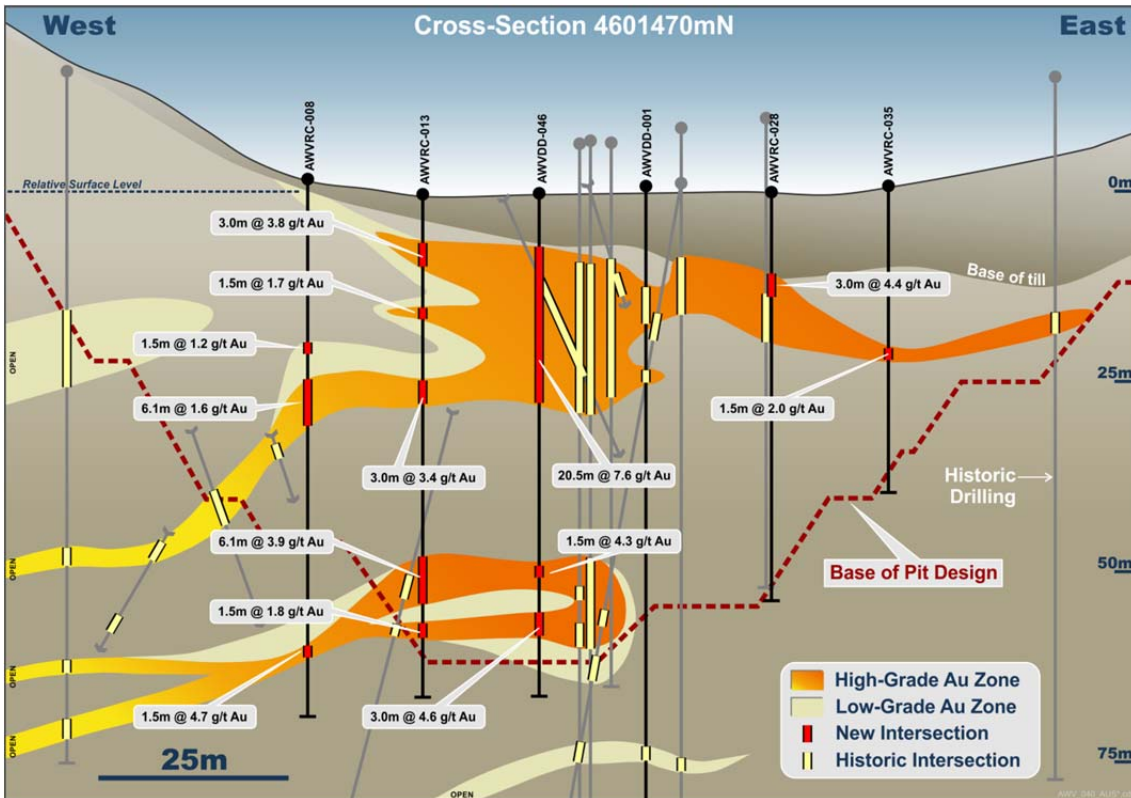
Figure 4: Cross section 4601470mN showing new drilling results at the 601 zone, South Sammy
